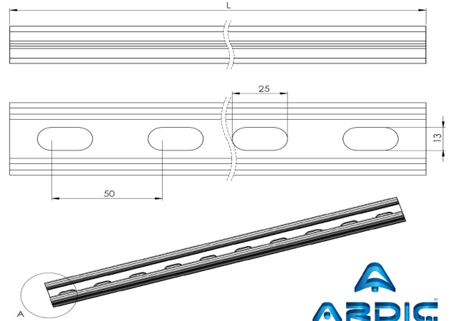
41X21 C PROFILE
