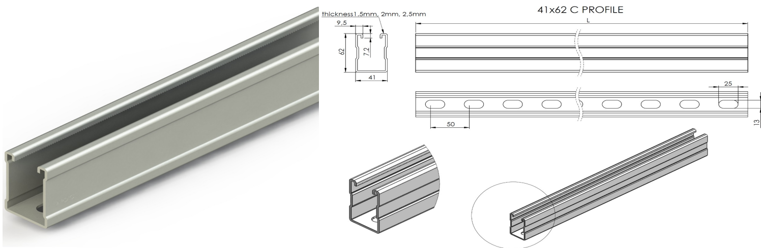
C Profile ( 1 Slot ) 62x41 L:3000mm T1,5mm PG
