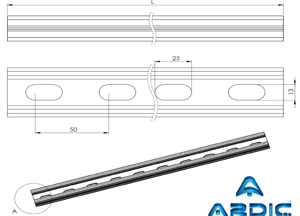
41X21 C PROFILE
