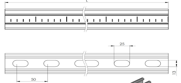
41X41 C PROFILE
