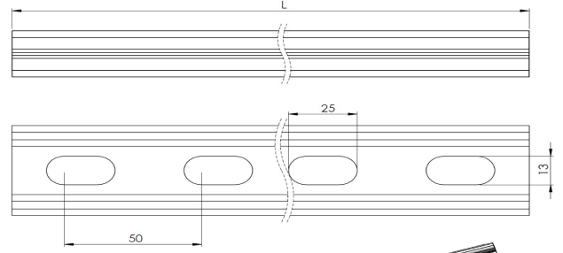
41X21 C PROFILE
